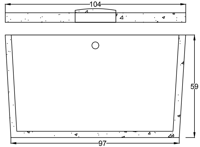
Tank End Profile
