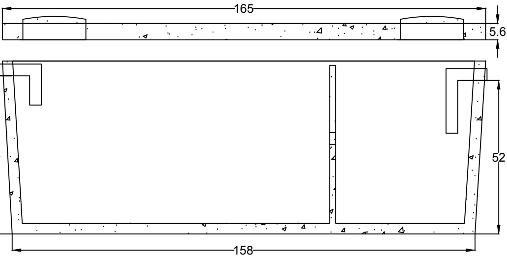
Tank Side Profile
